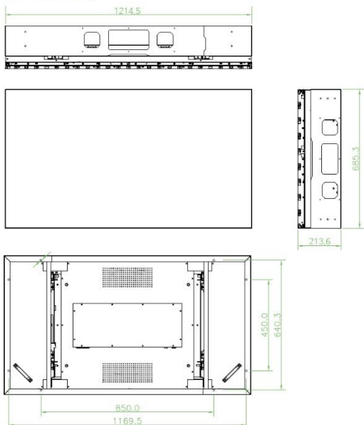
[Outside Dimension]
